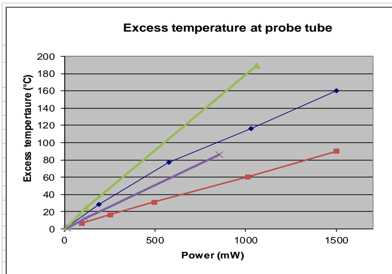
Overtemperature with loading of the measuring current circuit
